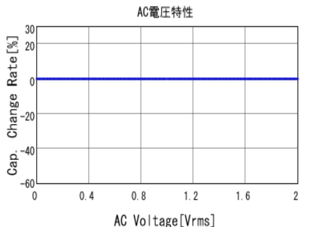
■RDE5C1H150J0P1H03B C-AC Voltage capchange, DC0V, 25.0
