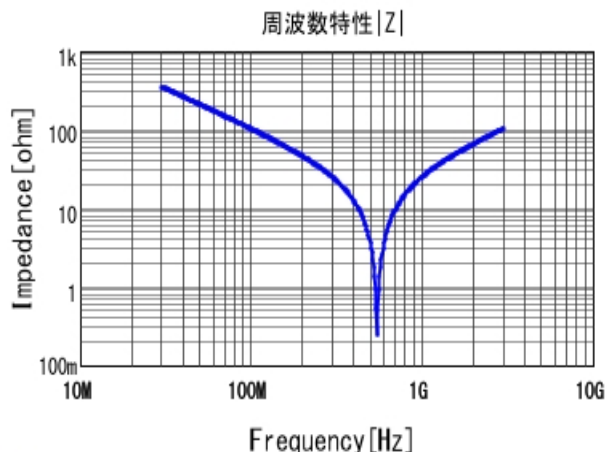
■RDE5C1H150J0P1H03B |Z| DC0V, 25degC
