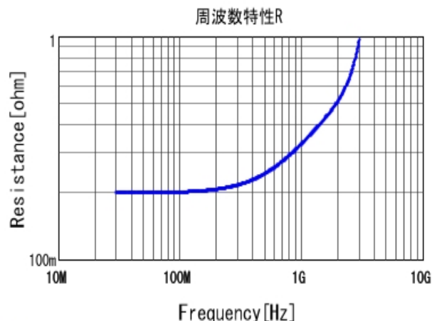
■RDE5C1H150J0P1H03B R DC0V, 25degC
