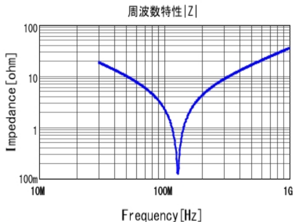
■RDE5C1H271J0P1H03B |Z| DC0V, 25degC
