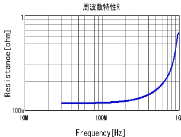
■RDE5C1H271J0P1H03B R DC0V, 25degC
