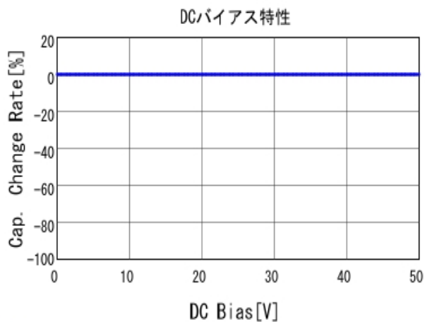
■RDE5C1H271J0P1H03B C-DC bias capchange, 25.0degC, AC1
