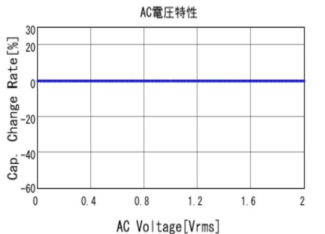
■RDE5C1H271J0P1H03B C-AC Voltage capchange, DC0V, 25.0
