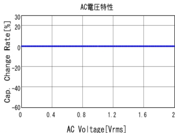
■RDE5C1H821J0K1H03B C-AC Voltage capchange, DCOV, 25.0
