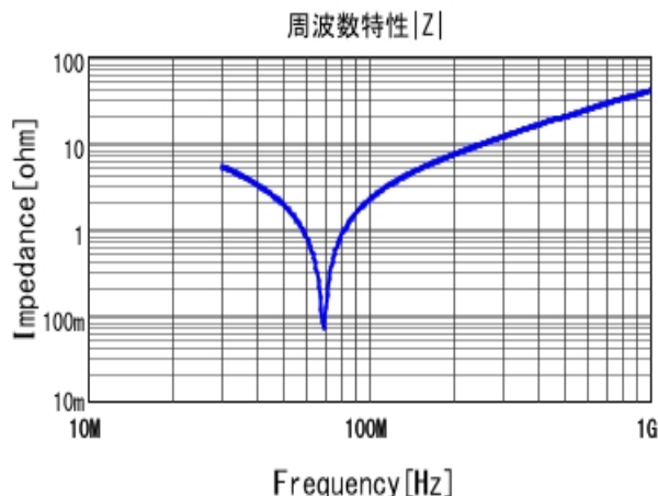
■RDE5C1H821J0K1H03B |Z| DCOV, 25degC
