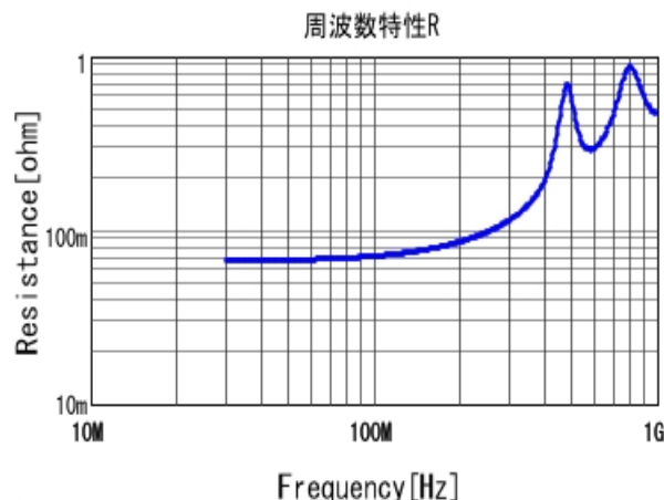
■RDE5C1H821J0K1H03B R DCOV, 25degC
