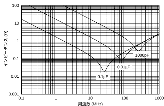
BΔ, RΔ特性：GRM15
