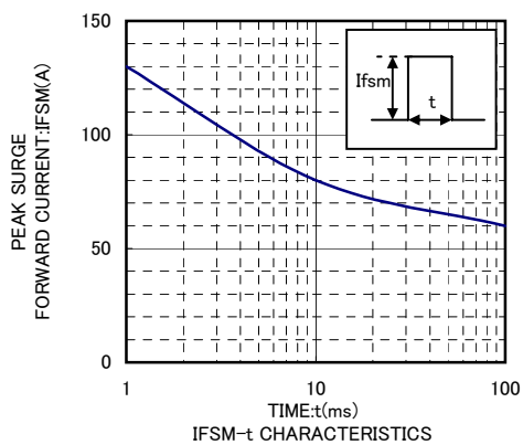
IFSM-t CHARACTERISTICS
