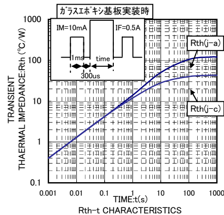
Rth-t CHARACTERISTICS
