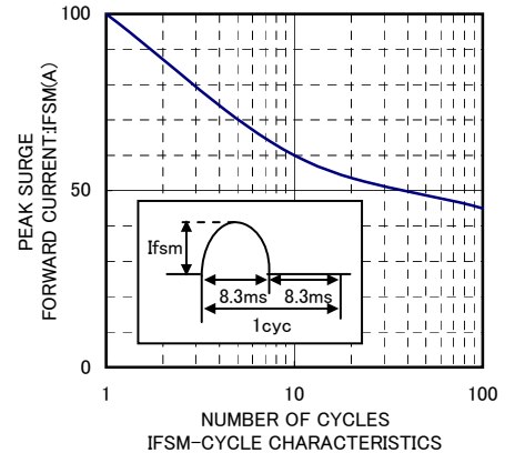
IFSM-CYCLE CHARACTERISTICS
