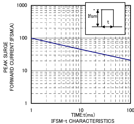
IFSM-t CHARACTERISTICS
