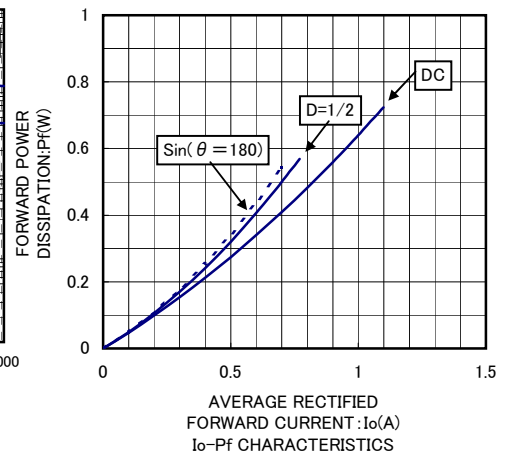
Io-Pf CHARACTERISTICS
