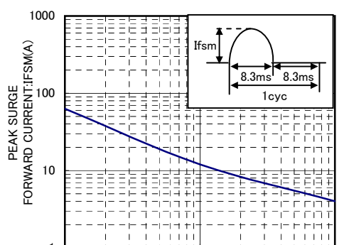
IFSM-CYCLE CHARACTERISTICS
