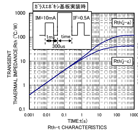
Rth-t CHARACTERISTICS
