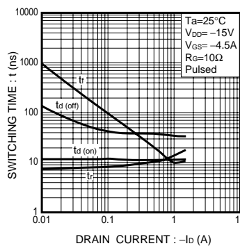
Fig.8 Switching Characteristics
