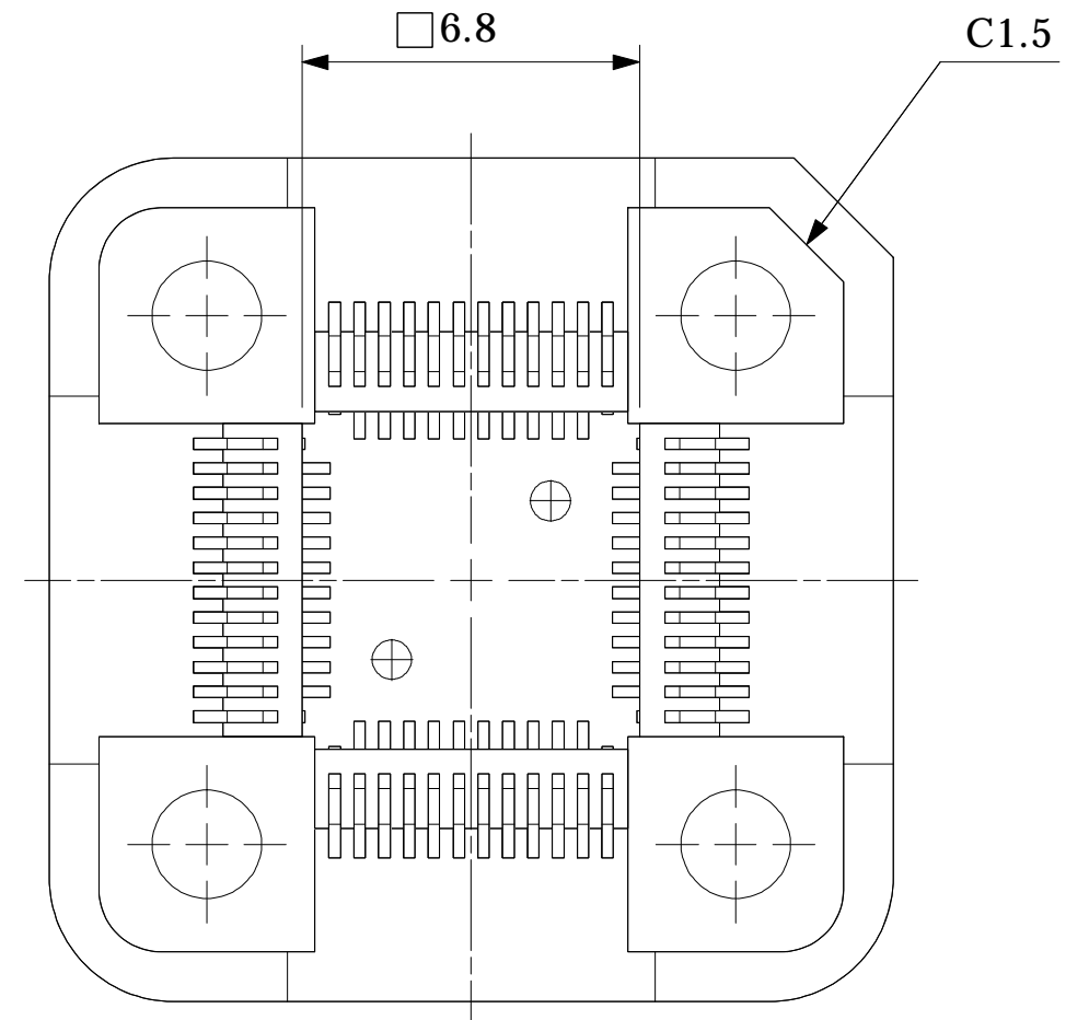
BOTTOM VIEW
