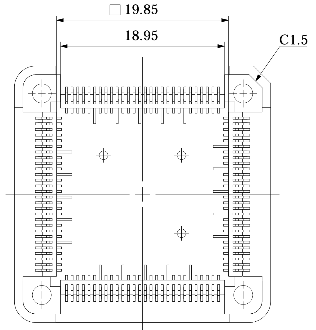
BOTTOM VIEW
