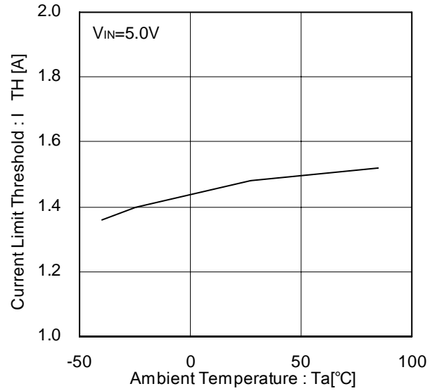
Figure 13. 過電流検出値
