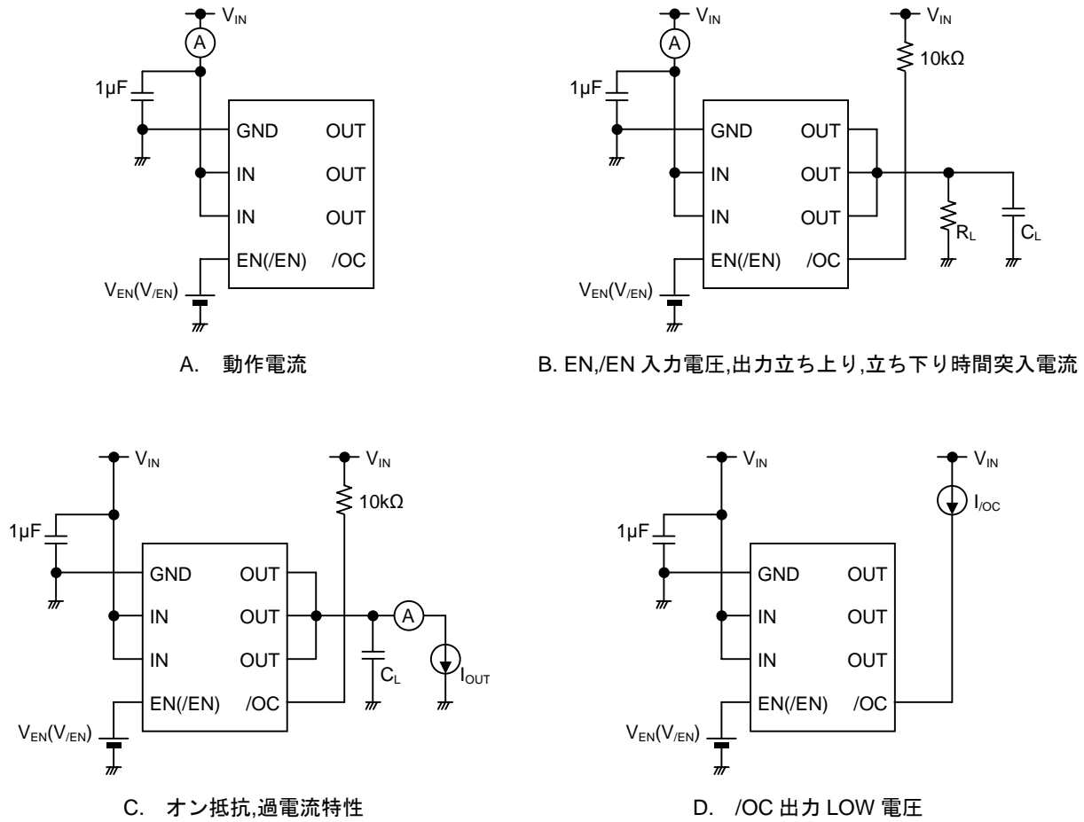
Figure 1. 測定回路
