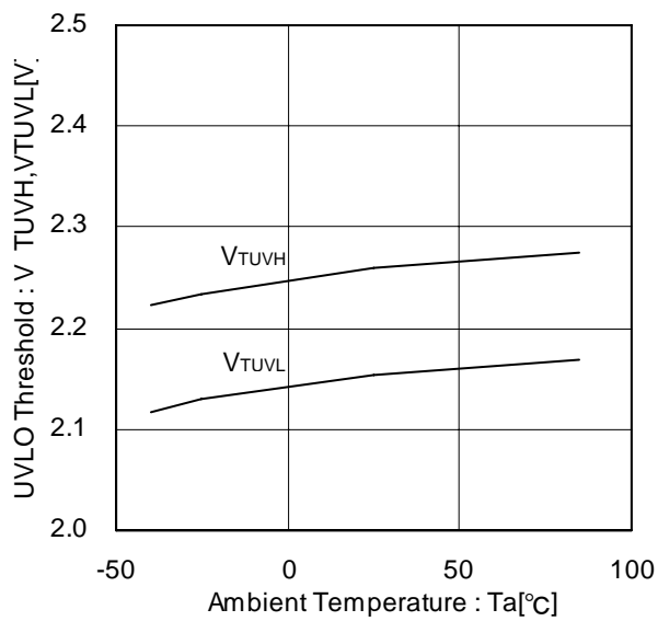
Figure 18. UVLO 検出電圧
