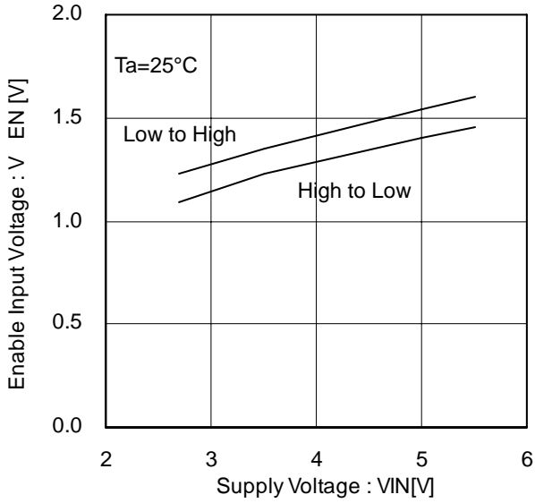
Figure 8. EN, /EN 入力電圧
